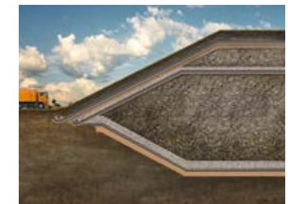
Landfill Construction
