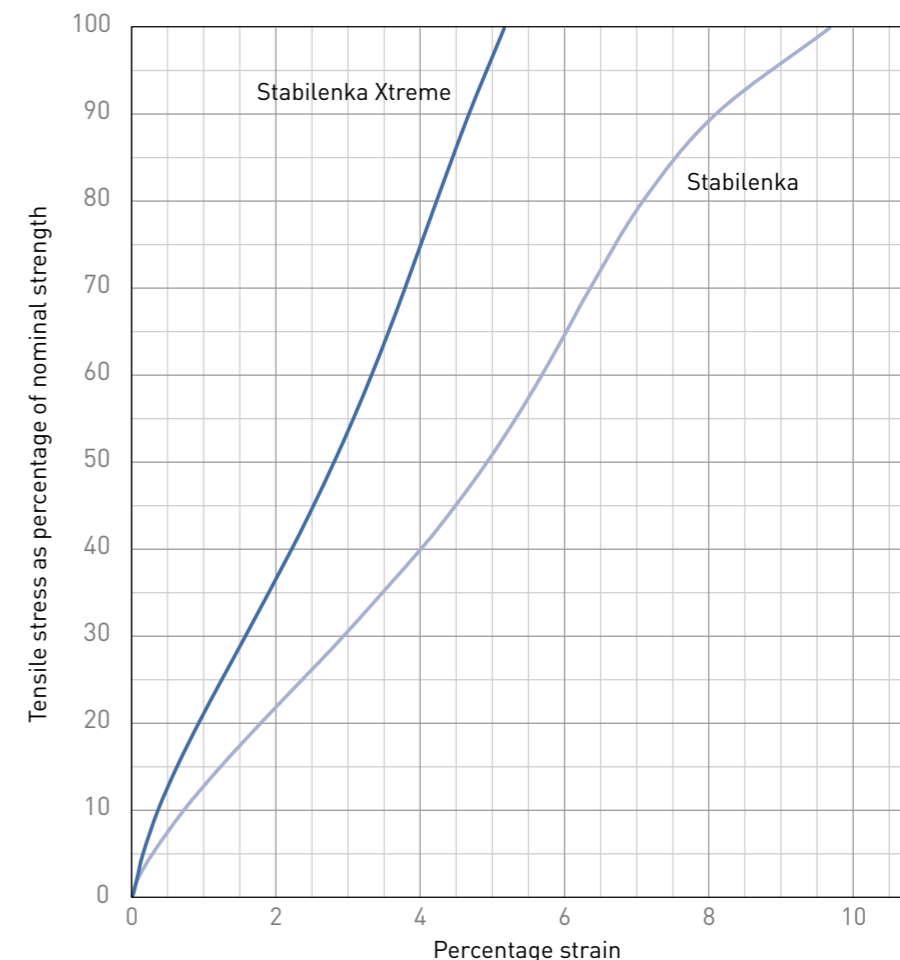
Specimen short term tensile stress-strain curves
